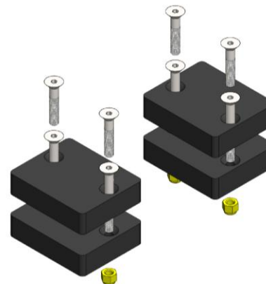
Figure 33: Bump-stops (1-2" tall stackable bump-stop options)
