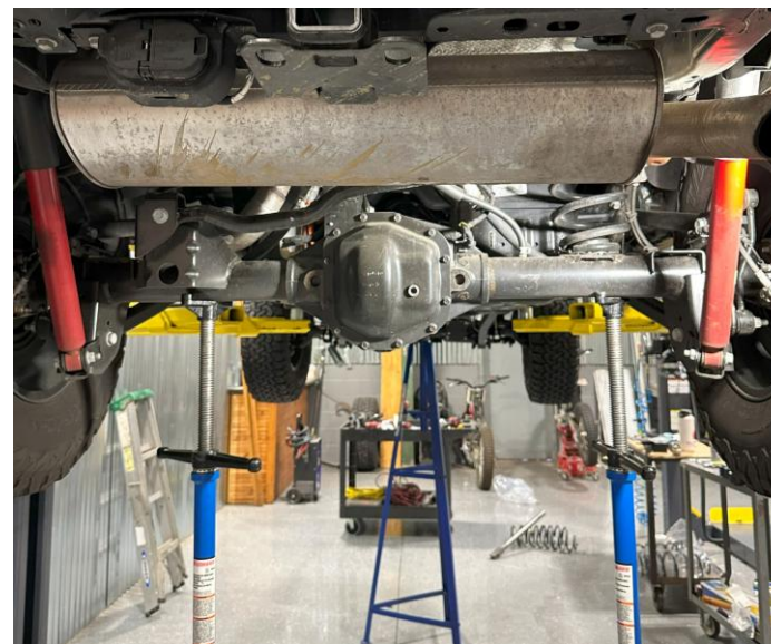
Figure 19: Vehicle rear axle supported by lift and jack stands
