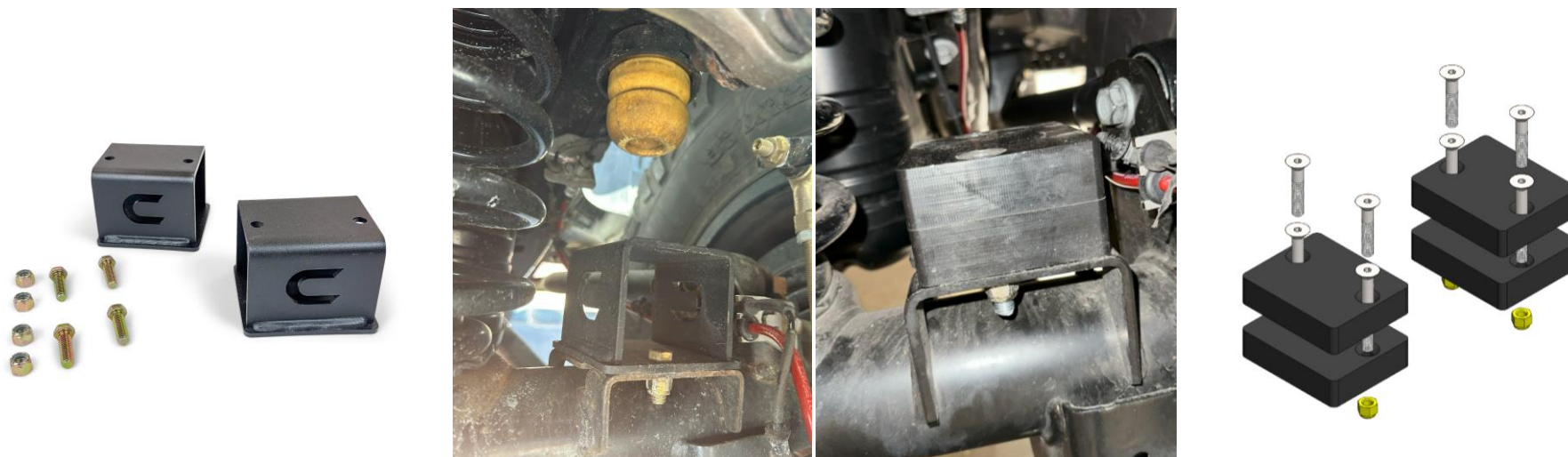
Figure 33: Bump-stops (3" tall and 1-2" tall stackable bump-stop options)
