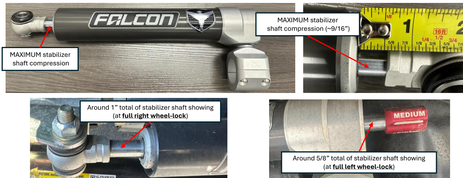
Figure 8b: Falcon Nexus EF 2.2 Stabilizer with max shaft compression and proper installation set-up
